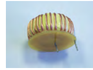
FR4 SPACER (COIL BASED-1)
