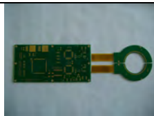
FLEXIBLE-RIGID - AE
